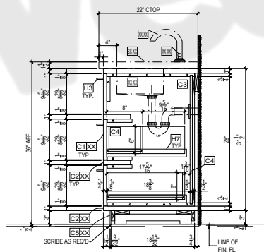
2 VERT. SECT. 11.0 SCALE: 1-1/2"=1'-0" REF: N/A
