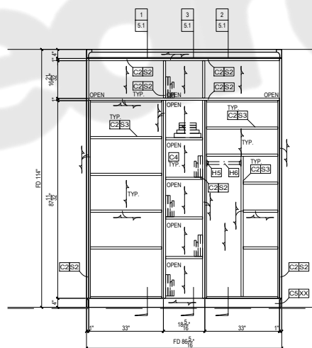
DETAIL SCALE: 1/4"=1'-0" REF: NA
