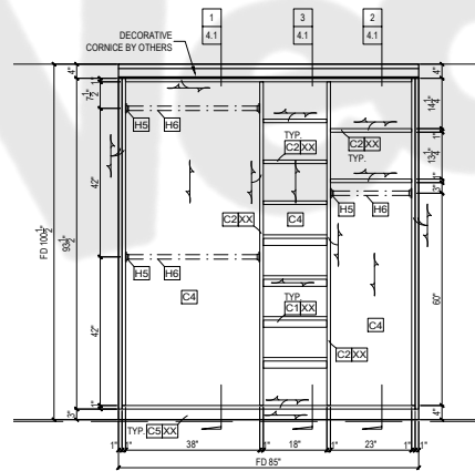
4 4.0 ELEVATION W/O DOOR @ MASTER CLOSET SCALE: 3/16"=1'-0" REF. -
