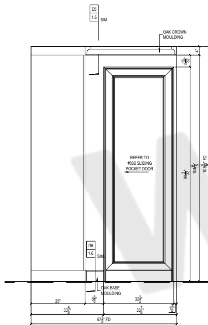
E 1.4 ELEVATION W/ DOOR @ PRIMARY ROOM SCALE: 1"=1'-0" REF: M2
