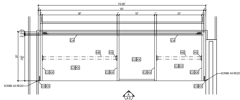
4 4.0 PLAN @ MASTER CLOSET SCALE: 1/32"=1'-0" REF. -
