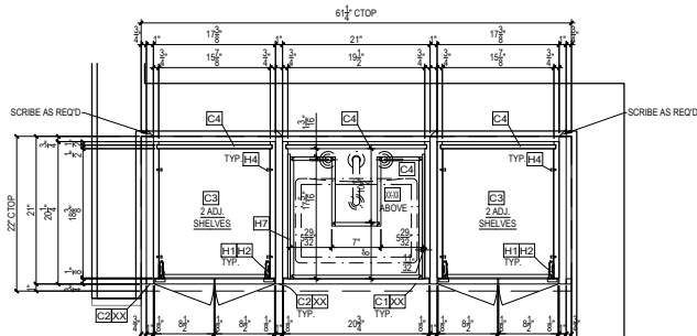
1 HORZ. SECT. 11.0 SCALE: 1-1/2"=1'-0" REF: N/A
