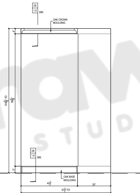
G 1.4 ELEVATION W/ DOOR @ PRIMARY ROOM SCALE: 1"=1'-0" REF: M2
