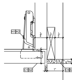
DETAIL SCALE: 1/4"=1'-0" REF: NA
