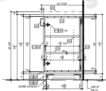
3 VERT. SECT. 11.0 SCALE: 1/4"=1'-0" REF: NA
